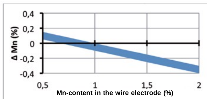
Pick-up/Burn-out Manganese
